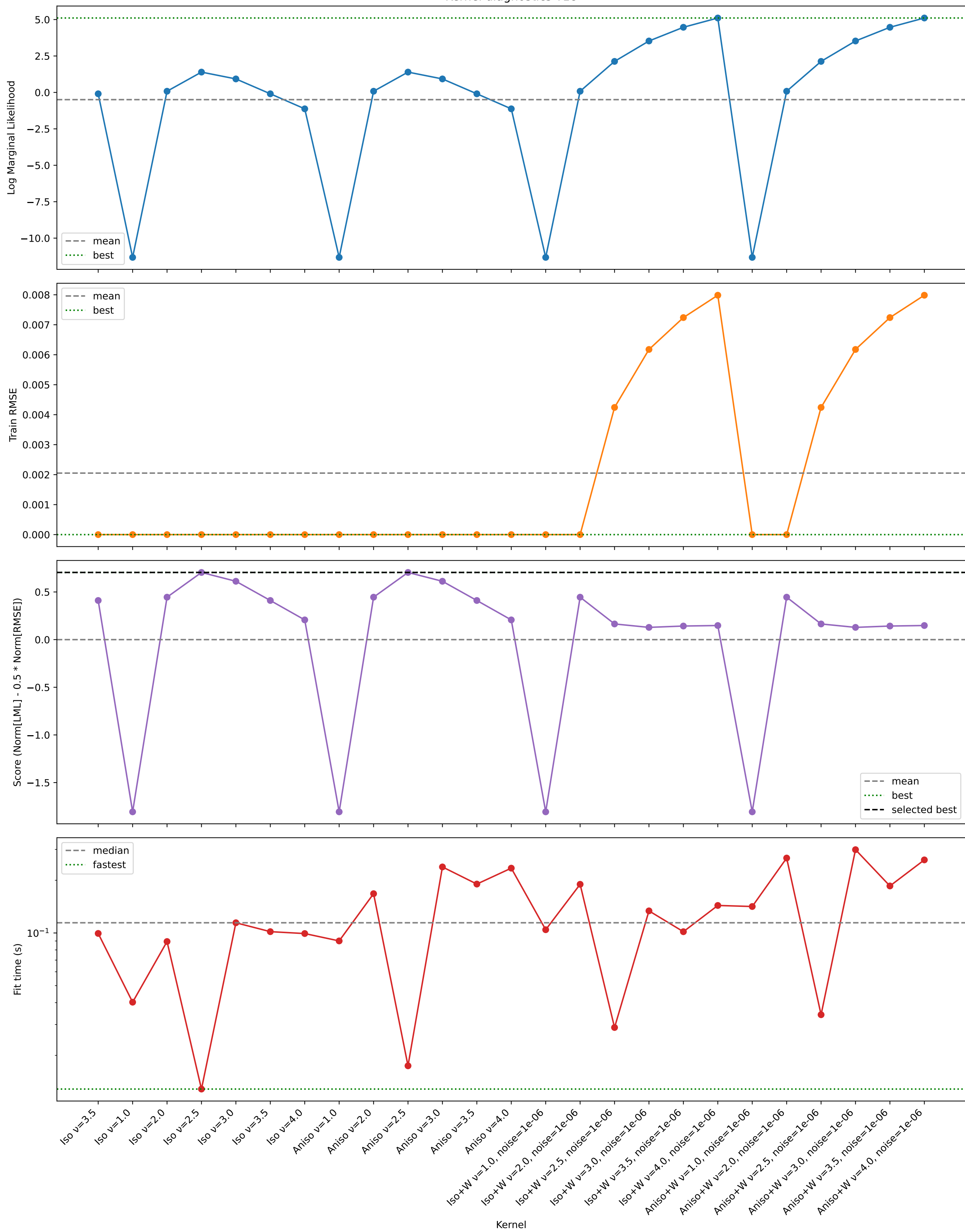
Kernel diagnostics T18
