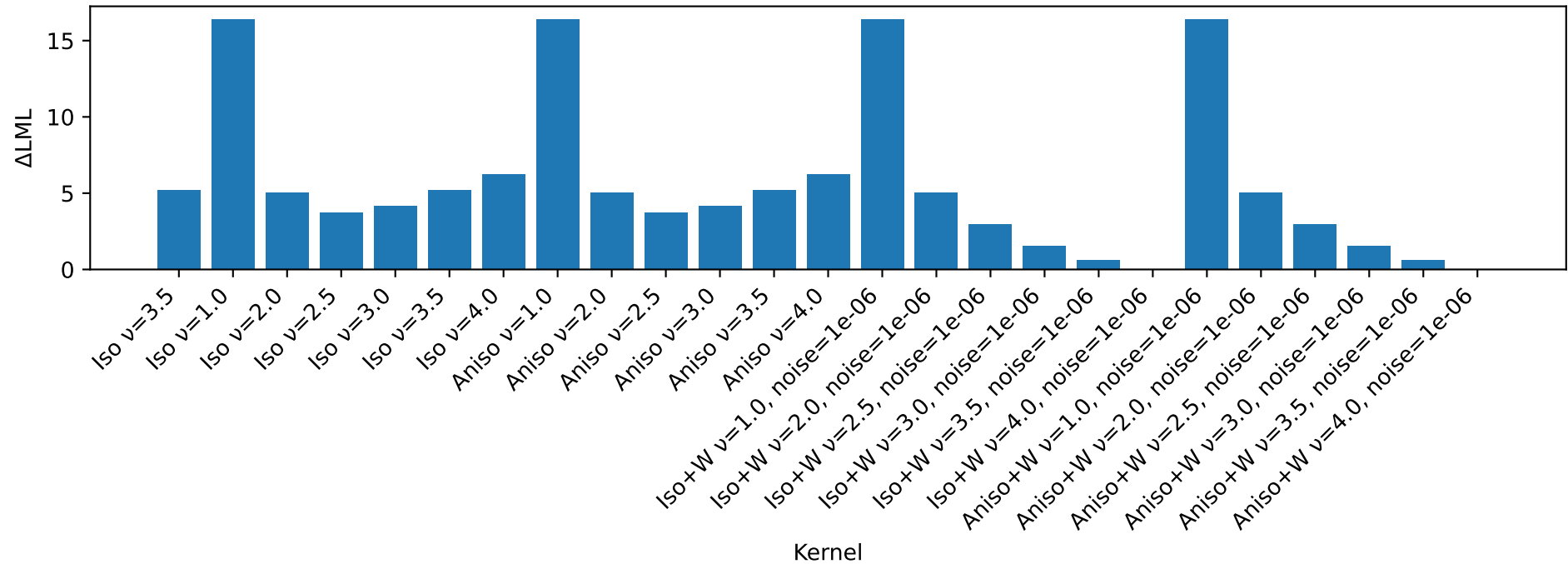
Difference from best LML (T18)
