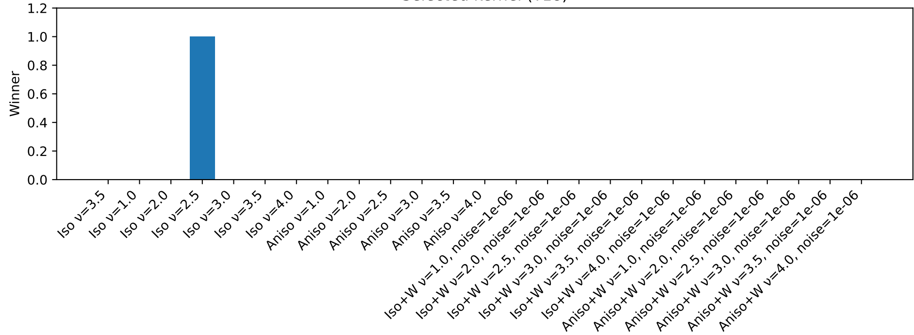
Selected kernel (T18)
